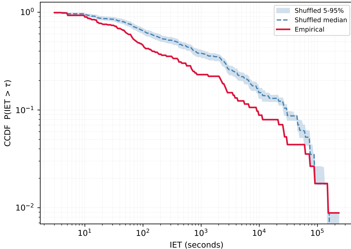
User 693274644 - Empirical vs Reshuffled | KS=0.207 p=0.000
